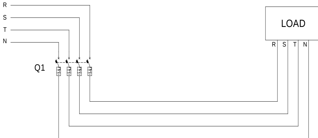
Pre-installation diagram without ICO-F system
