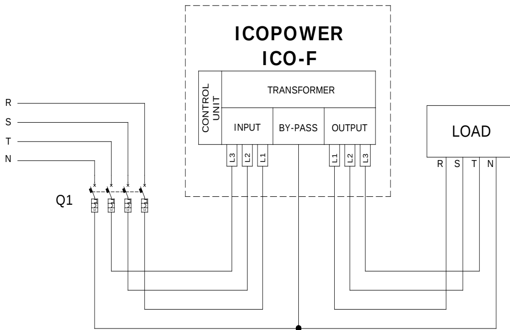
Post-installation diagram with ICO-F system
